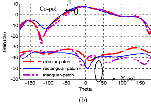
Figure 6. Simulated radiation patterns of the different hybrid antennas including co- and cross-polarization patterns at 8 GHz : a) H-plane, b) E-plane.
