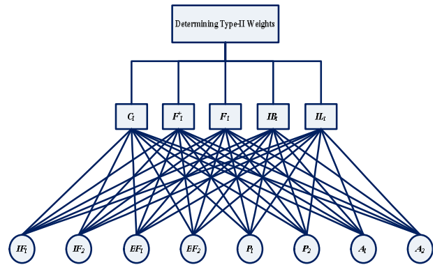
Figure 2. The hierarchical graph for determining type-II weights
