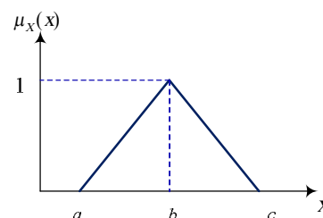
Figure 1. Membership function of triangular fuzzy number
