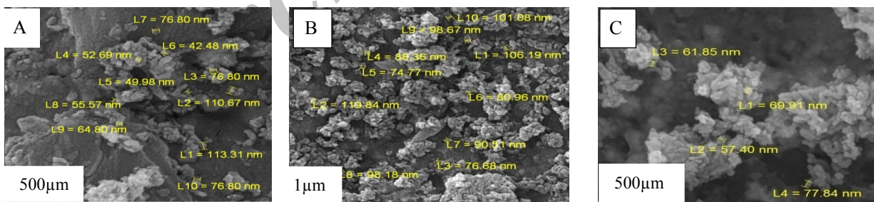
Figure 6. SEM micrographs of the obtained powders (a) PLW (b) NaOH (c) Thermal
