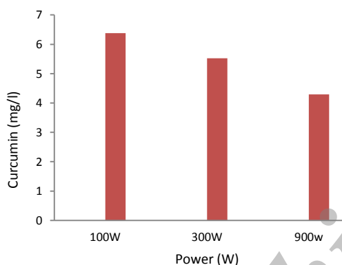
Figure 3. Effect of microwave power on extraction of curcumin from turmeric cell (irradiation exposure time 2 min and particle mesh size of 70)
