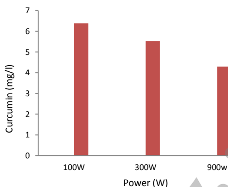
Figure 3. Effect of microwave power on extraction of curcumin from turmeric cell (irradiation exposure time 2 min and particle mesh size of 70)
