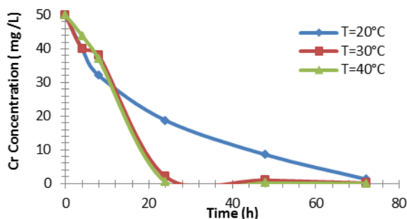
Figure 3. Effect of incubation time on Cr(VI) reduction at temperatures of 20, 30 and 40 °C [conditions: inoculum volume of 5 mL, pH 7, initial Cr(VI) concentration of 50 mg/L]
