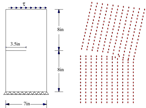
Figure 12. (a) Ggeometry and loading of an edge cracked plate under Mixed mode; (b) displaced geometry of plate in the final step of analysis
