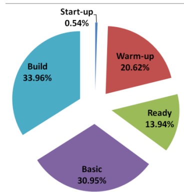
Figure 6. Energy demand during fabrication of 9000 mm3 volume part.
