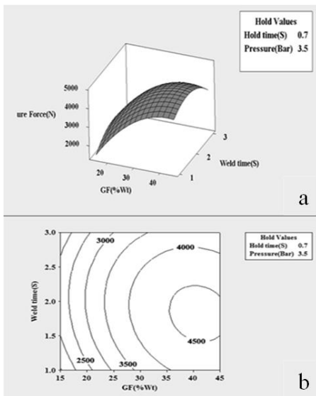
Figure 4a. Surface response of the effect of GF% - welding time on weld failure force 4b. Two-dimensional plot
