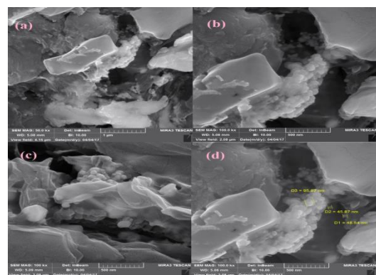
Figure 2. SEM images of (a-d) Ag/GO nanocomposites
