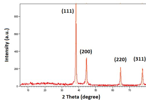
Figure 1. XRD patterns of Ag/GO nanocomposite
