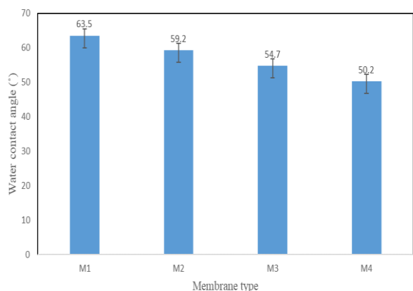
Figure 3. Water contact angle of the produced membranes
