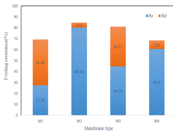
Figure 9. Fouling resistance ratio of Ag/GO-PES ultrafiltration membranes
