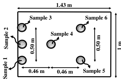
Figure 14. Plan of test box containing sampling molds (Uniformity tests in the horizontal direction)
