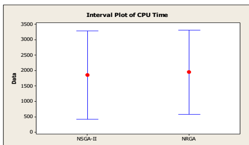
Figure 8. The intervals plot of CPU Time
