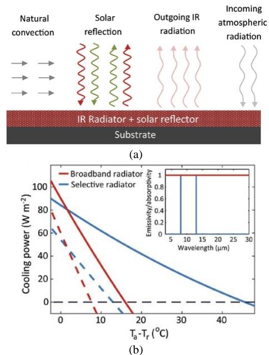
Figure 1. a) Theoretical model of the radiative cooling material which clarifies fundamental parts required for radiative cooling. b) Performance of broadband and selective radiators, inset refers to ideal radiators [2]
