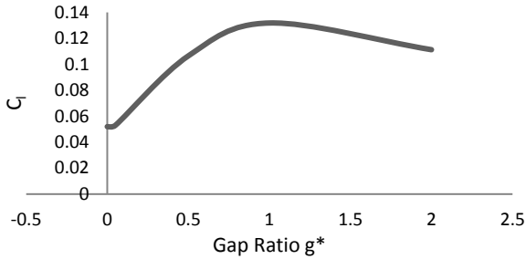
Figure 5. C_l variation with gap ratio at a 30° angle of attack
