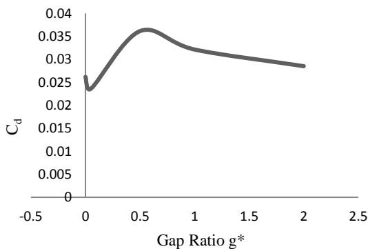
Figure 7. C_d variation with gap ratio at a 15° angle of attack
