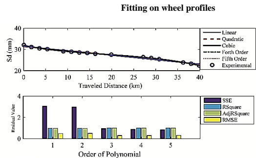
Figure 7. The critical wheel wear behavior from experimental data obtained through field data recording in Southern line of Iran’s Railway System
