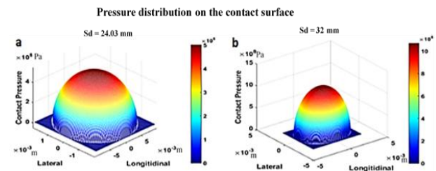
Figure 11. A 3D schematics of the contact ellipse showing the values of pressure on the contact surface for: (a) Sd=24.03 mm (Max.) and (b) Sd=32 mm (Min.). The maximum pressure occurs at the center of the ellipse
