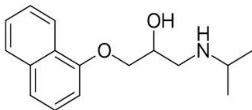
Figure 1. Chemical structure of propranolol.
