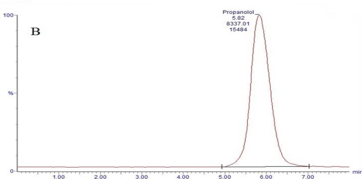
Figure 3. The chromatogram exhaled breath condensate sample was taken from a patient receiving propranolol.
