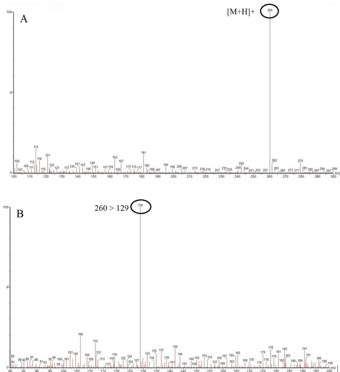
Figure 2. A) Full scan mass spectrum and B) parent to daughter mass spectrum of spiked propranolol in exhaled breath condensate.
