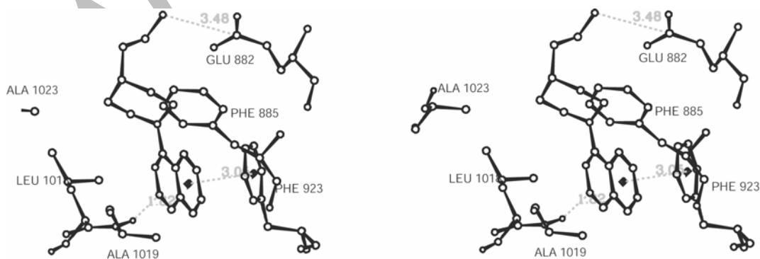
Figure 6. Stereo presentation of the residues interacting with the substrate P7 docked into the active site. Phe 655 and hydrogen atoms are not shown for clarity except for the amide proton of Ala1019 where a hydrogen bond is formed between enzyme and substrate.
