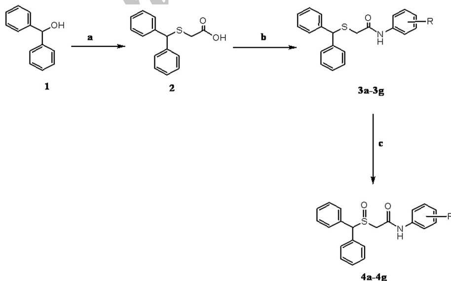
Scheme 1 Synthesis of target compounds 4a-4g (R: (a) = H, (b) = 3-Cl, (c) = 4-Cl, (d) = 4-Et, (e) = 3,4-Cl, (f) = 4- \text{NO}_2 , (g) = 4-Br), Reagents and conditions: (a) Thioglycolic acid, TFA, 3 h; (b) appropriate amine, EDC, HOBt; (c) appropriate amide, \text{H}_2\text{O}_2 , acetic acid.
