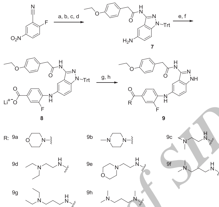
Figure 3 Synthetic scheme for compound 9a to 9h. Reagents and experimental conditions: a) \text{H}_2\text{NNH}_2 , n -BuOH, reflux, b) i) p\text{-C}_2\text{H}_5\text{OC}_6\text{H}_4\text{CH}_2\text{COCl} , THF, reflux, ii) 2N NaOH c) TrtCl, \text{Et}_3\text{N} , \text{CH}_3\text{CN} , reflux, d) Pd/C, \text{H}_2 , MeOH/DCM, e) 2-F-4-EtO 2 CC 6 H 3 Br, Pd 2 (dba) 3 , (R)-BINAP, NaOBu- t , toluene, reflux, f) LiOH, THF:H 2 O:MeOH (3:1:1), reflux, g) RH, EDC, HOBT, DMF, h) TFA, DCM.
