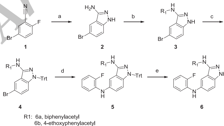
Figure 2 Synthetic scheme for compound 6a and 6b . Reagents and experimental conditions: a) H 2 NNH 2 , n -BuOH, reflux, b) i) 4-C 2 H 5 OC 6 H 4 CH 2 COCl (or 4-PhC 6 H 4 CH 2 COCl), THF, reflux, ii) 2N NaOH, c) TrtCl, K 2 CO 3 , CH 3 CN, reflux, d) 2-FC 6 H 4 NH 2 , Pd 2 (dba) 3 , (R)-BINAP, NaOBu- t , toluene, reflux, e) TFA:Phenol:H 2 O:TIPS (88:5:5:2), DCM.
