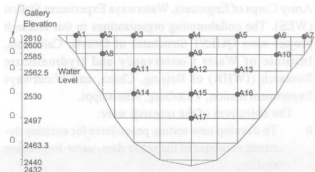
Figure 3. Accelerometers mounted on dam crest and in galleries.
