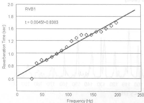
Figure 14. Variation of reverberation time with frequency.
