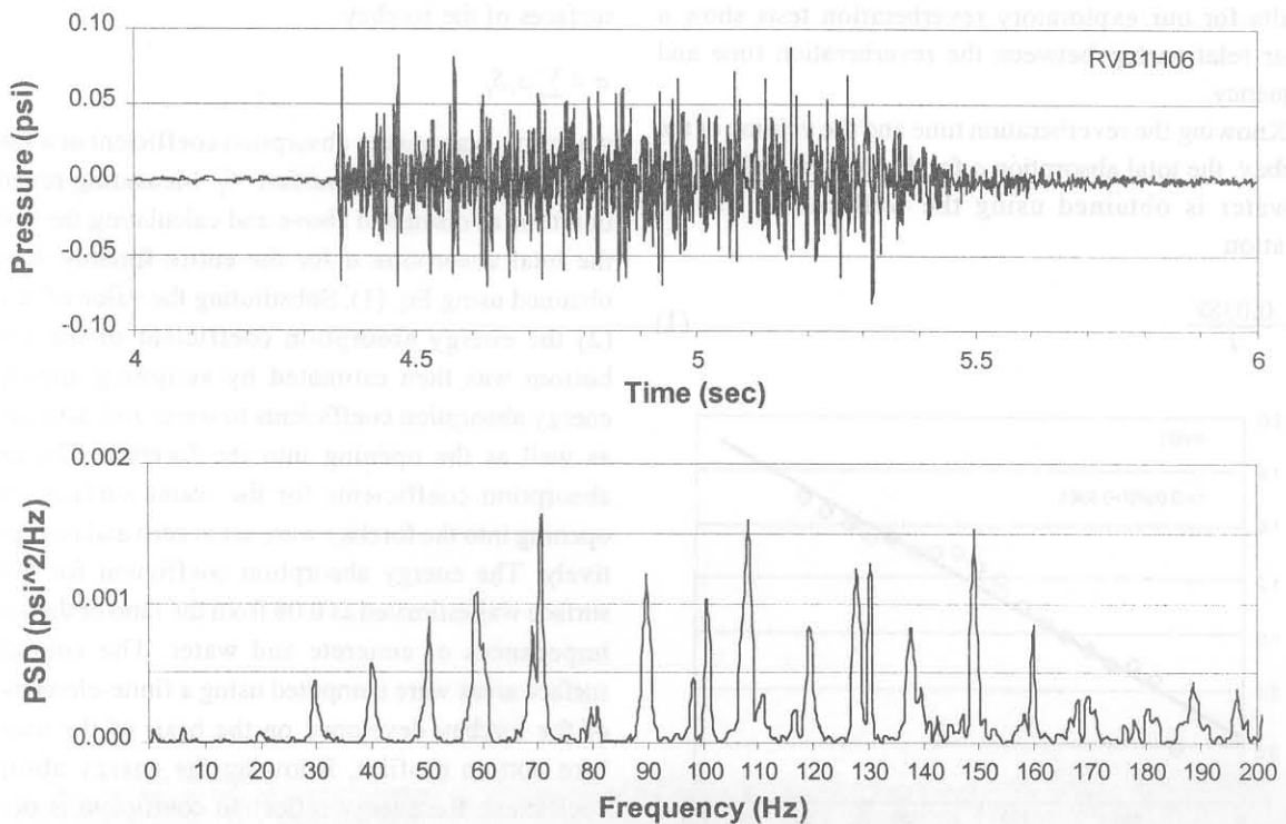
Figure 12. Recorded pressure and computed PSD function at forebay entrance due to reverberation test shot with 100ms delay.
