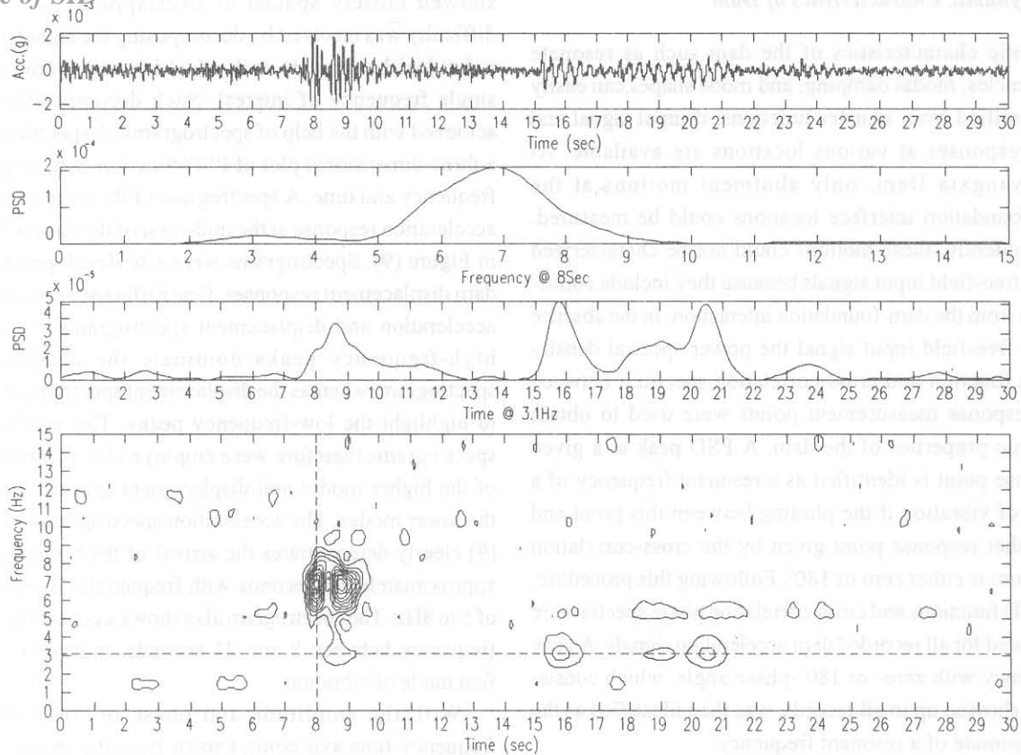
Figure 10. 2D spectrogram of recorded dam acceleration for 100kg charge.
