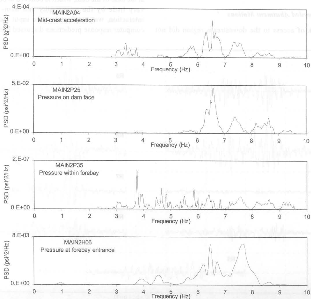
Figure 7. PSD of recorded dam acceleration and water pressures.
