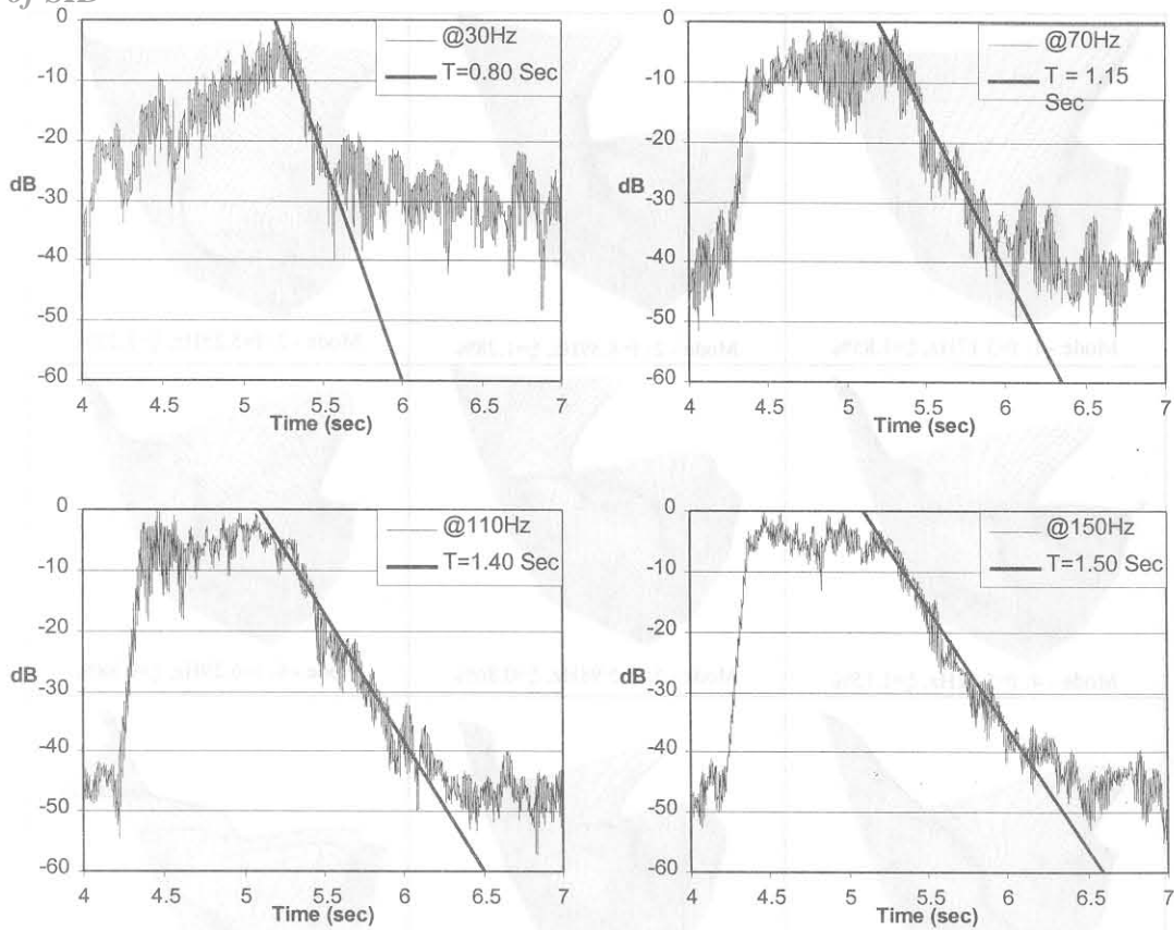
Figure 13. Reverberation time at various frequency bands.
