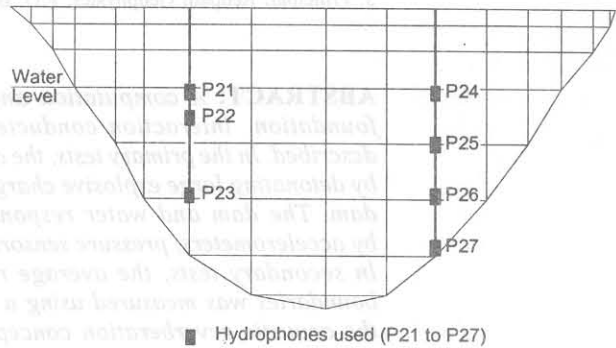
Figure 2. Hydrophones suspended on face of dam.
