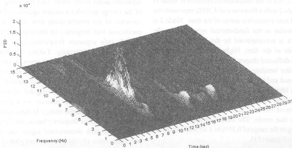
Figure 9. 3D spectrogram of recorded dam acceleration for 100kg charge.
