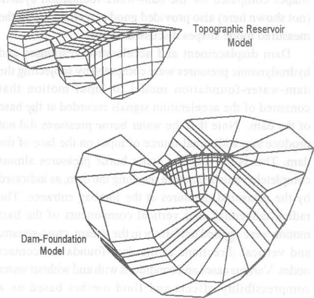
Figure 15. Perspective view of dam-water-foundation model.
