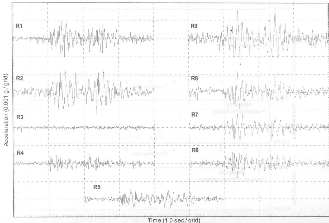
Figure 8. Seismograph radial accelerations at dam-foundation interface due to 300kg charge.
