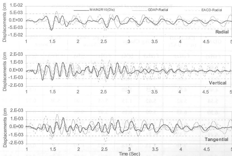
Figure 16. Comparison of measured and predicted crest displacements.
