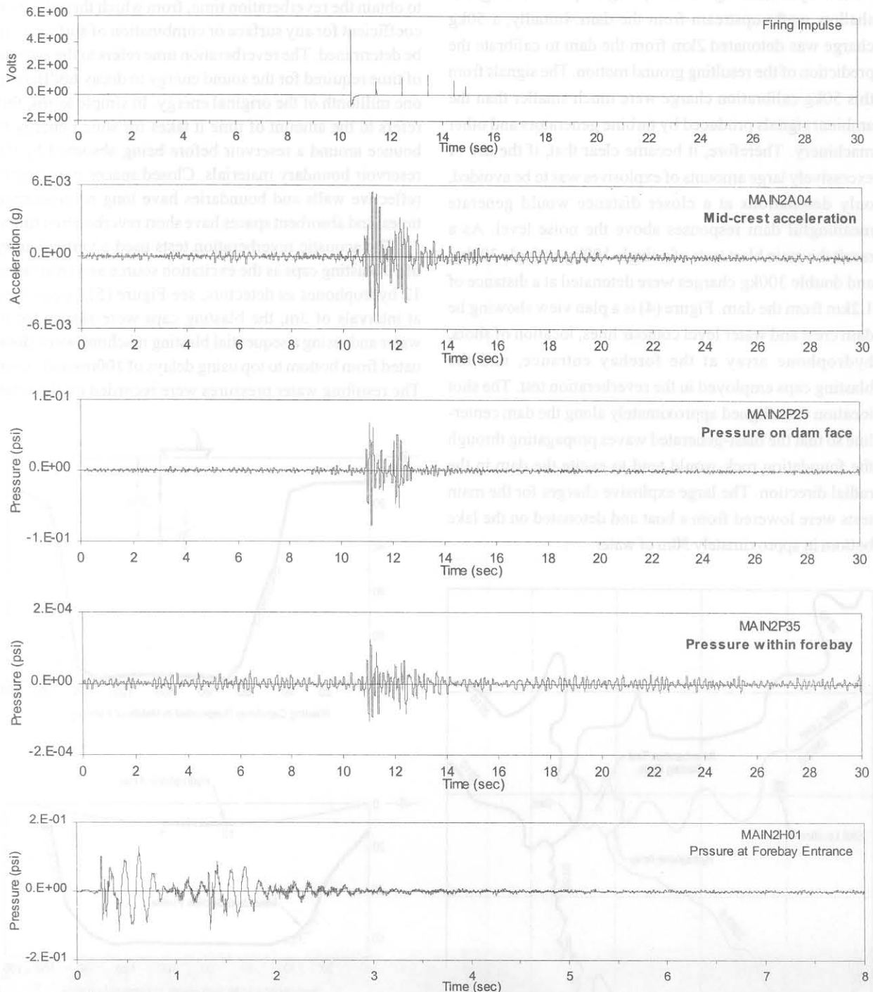
Figure 6. Examples of recorded firing impulse, dam acceleration, and water pressures for single 300kg charge.
