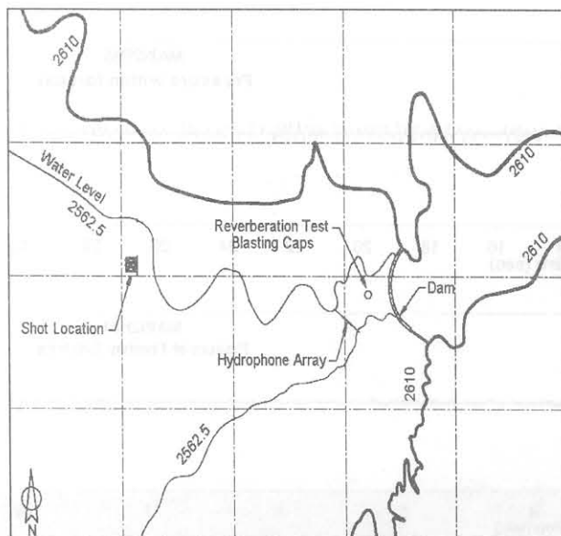
Figure 4. Plan view of Longyangxia dam and its retained water.
