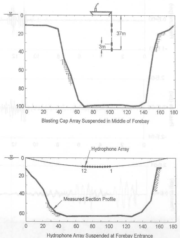
Figure 5. Acoustic reverberation test setup.
