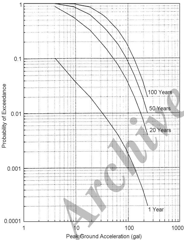
Figure 8. Curves of probabilities of exceedence in 1, 20, 50, 100 years at Kowloon site ( 114^{\circ}10'E, 22^{\circ}19'N ).
