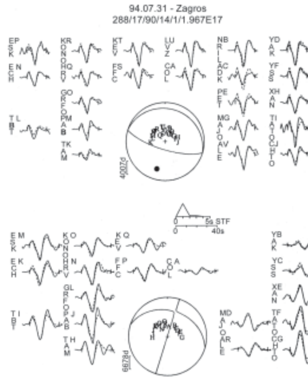
Figure 2. Minimum misfit solution for the event of 31 July 1994 in the Zagros. The values beneath the event header give strike, dip, rake, depth in km and seismic moment (in units of Nm). This solution was calculated using velocity model consisting of a 10km thick layer with V_p=6.0\text{ km s}^{-1} , V_s=3.45\text{ km s}^{-1} , \rho=2.78\text{ g cc}^{-1} over a half space with V_p=6.8\text{ km s}^{-1} , V_s=3.92\text{ km s}^{-1} and \rho=2.91\text{ g cc}^{-1} . The upper sphere shows the P wave radiation pattern and the lower sphere the SH radiation pattern. Both are lower-hemisphere projections. The station code by each waveform is accompanied by a letter corresponding to its position in the focal sphere. The positions are ordered clockwise by azimuth. The solid lines are the observed waveforms, the dashed lines are the synthetic waveforms. The inversion window is marked by solid bars at either end of the waveform. P and T axes are represented by solid and open circles respectively on the P-wave radiation pattern. The source time function is shown below the P focal sphere, with the waveform time scale below it. This figure was modified from Maggi et al [11] Figure (2).
