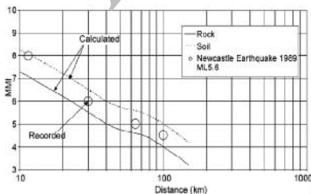
Figure 6. Comparisons of recorded and calculated MMI from the 1989 Newcastle Earthquake.
