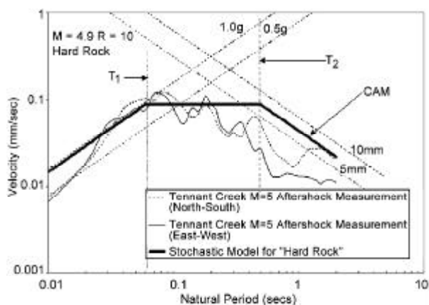
Figure 7. Response spectra for M4.9 Tennant Creek aftershock.
