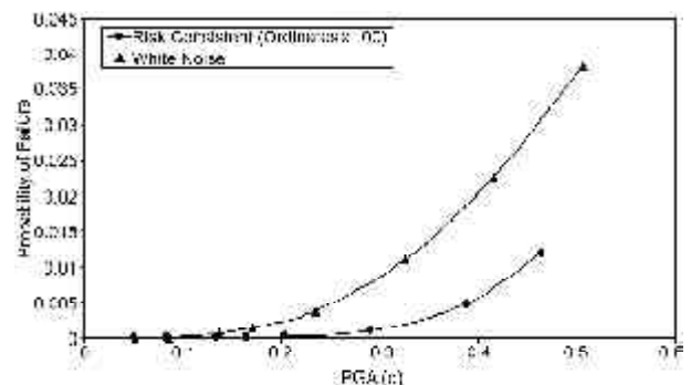
Figure 10. Comparison between fragility curves for different input response spectra.
