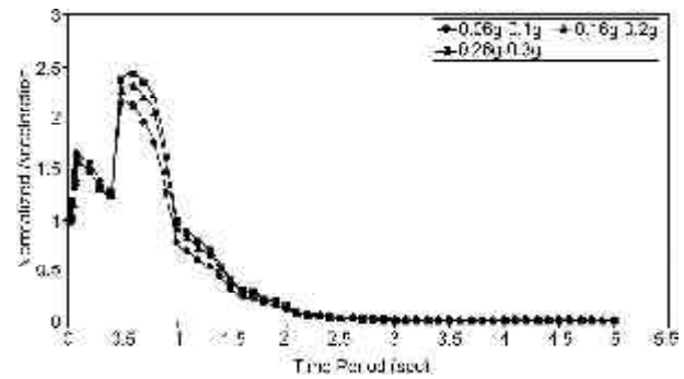
Figure 2. Normalized response spectrum at bedrock.
