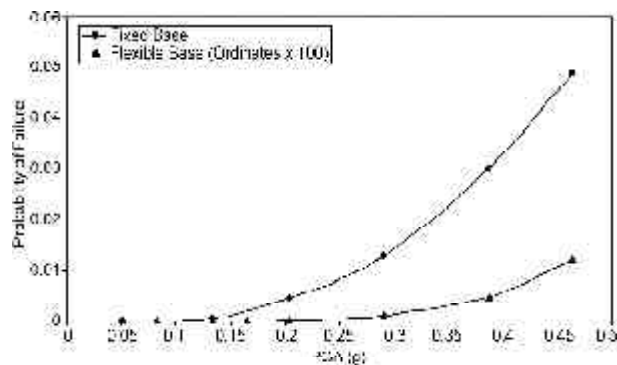
Figure 6. Comparison between fragility curves for flexible and fixed base conditions.
