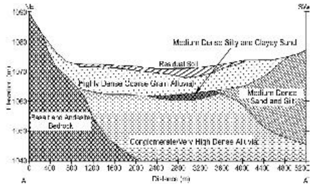
Figure 5. Geological profile of section A-A' shown at Figure (1).
