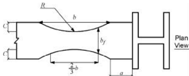
Figure 2. Geometric parameters of RBS connection.
