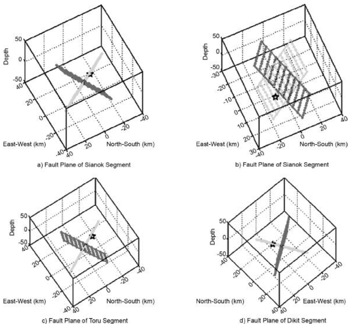
Figure 4. Fault plane identification of 4 events that occurred at 3 segments of SFZ, see Table (6). Two nodal planes pass through the centroid (LAT=0 and LON=0), both according to the MT solution of this paper, and the hypocenters for all events. These are the favorable cases, with hypocenter in one of the nodal planes, thus indicating the fault plane.
