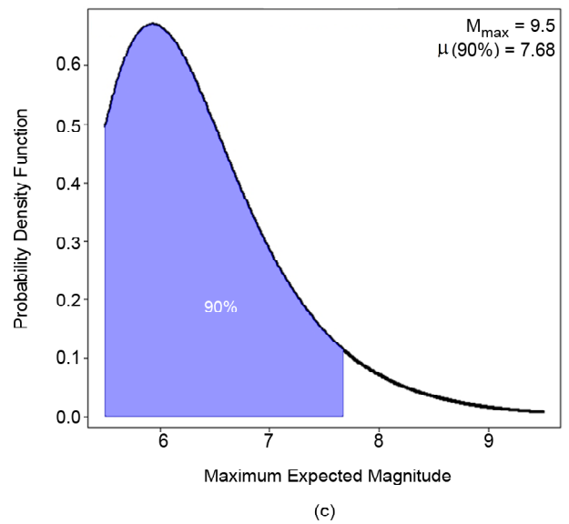
Figure 3. Bayesian posterior density function of \mu_i and T_f=30 years for the Azerbaijan seismotectonic zone and three choices of M_{max} : (a) M_{max} = 8.5 , (b) M_{max} = 9.0 , and (c) M_{max} = 9.5 . The shaded area corresponds to the 90% confidence interval.
