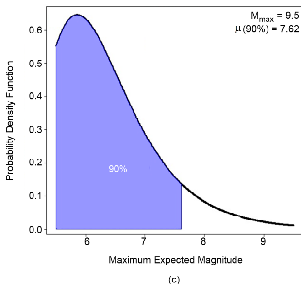
Figure 2. Bayesian posterior density function of \mu_i and T_f=30 years for the Alborz seismotectonic zone and three choices of M_{max} : (a) M_{max} = 8.5 , (b) M_{max} = 9.0 , and (c) M_{max} = 9.5 . The shaded area corresponds to the 90% confidence interval.
