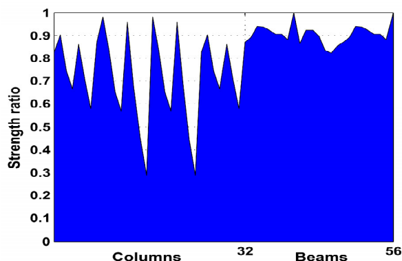
Fig. 10. Strength ratio in the members of the optimum solution obtained by HBB-BC for the three bay, eight-story reinforced concrete frame
