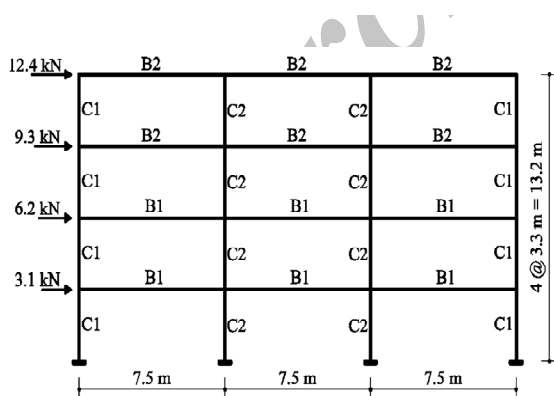
Fig. 5. Three-bay, four-story reinforced concrete frame
