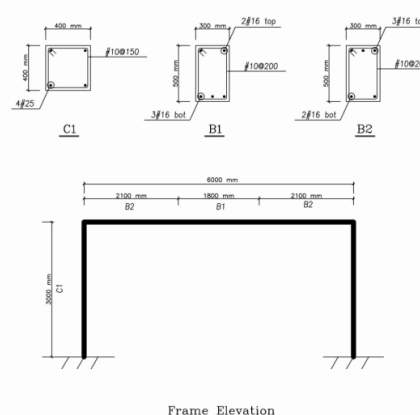
Fig. 5. Geometry and configuration of modeled frame
