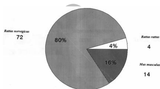
Fig. 1. Frequency and percentage of different species of rodents trapped in Ahvaz (1999-2000)
