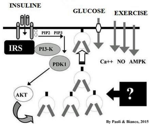
Fig. 1: Intracellular transport mechanisms of glucose
