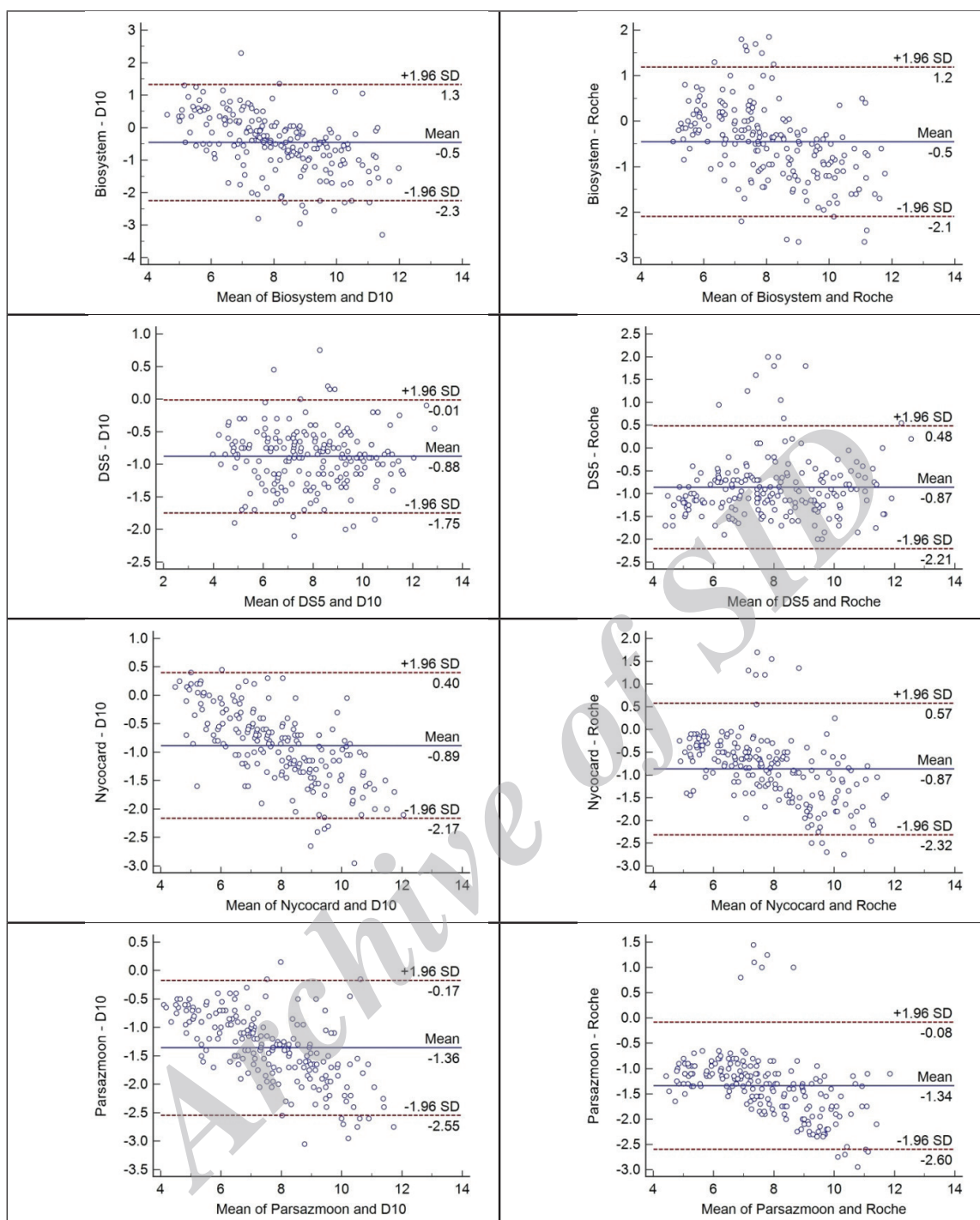
Figure 1. Bland-Altman plot examination for calculating absolute difference between methods.
