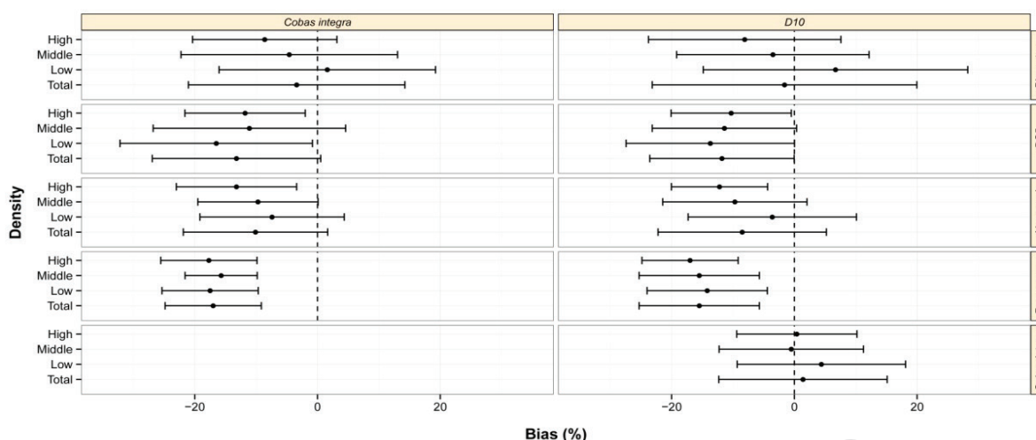
Figure 2. The percentage of bias with upper and lower bound in the different methods.
