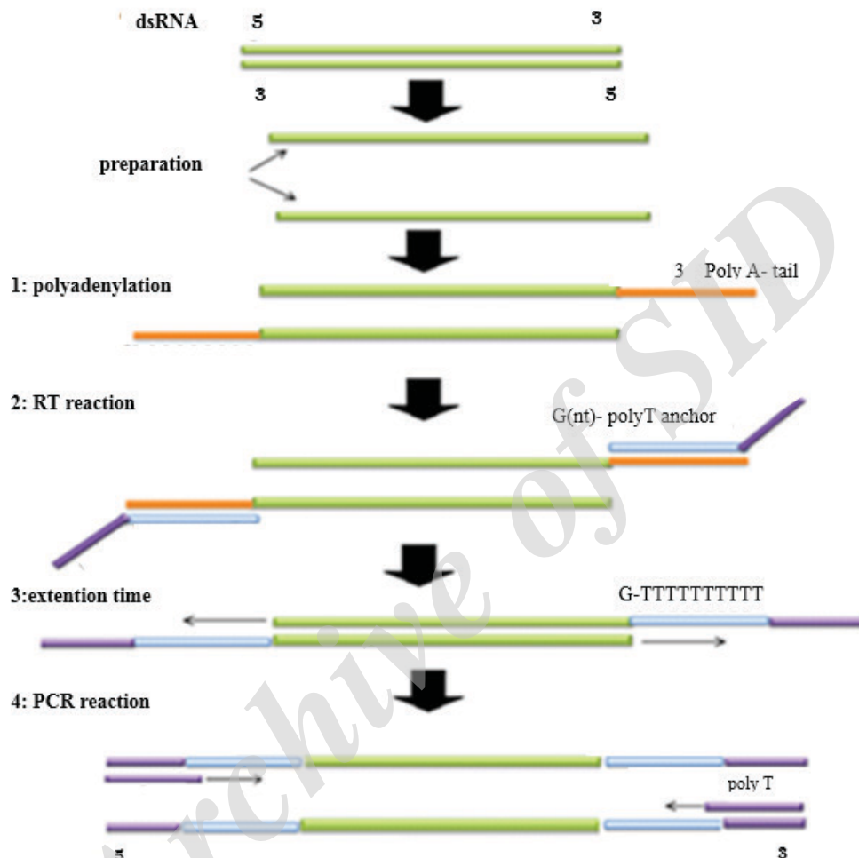
Figure 1. Schematic picture showing the four main steps of Poly (A)-Tailed Universal Reverse Transcription PCR method.
