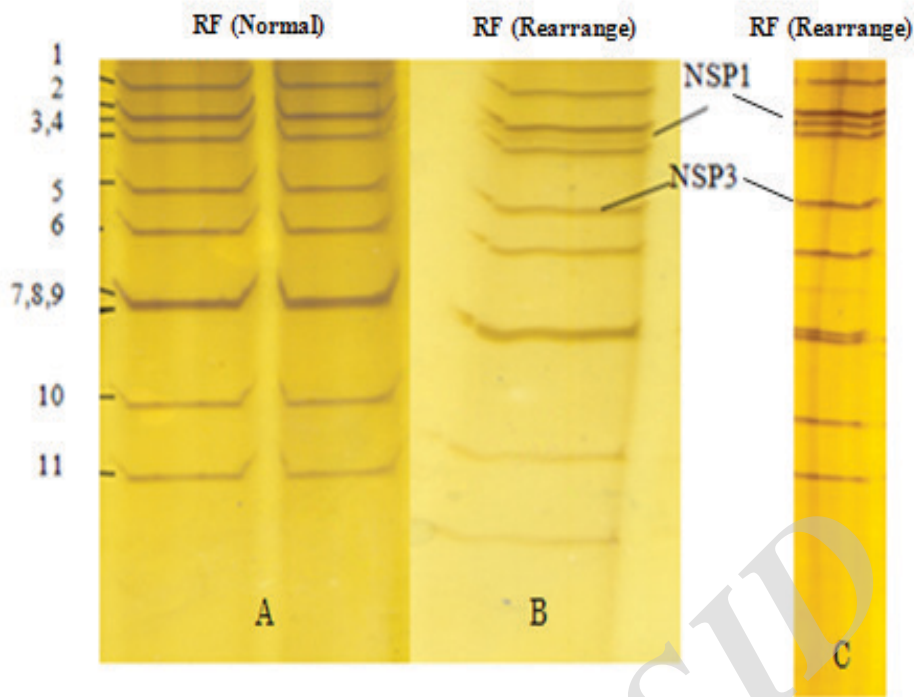
Figure 2. Normal (A) and rearranged (B, C) electrophoretic patterns of rotavirus dsRNA in 10% polyacrylamide gels and silver staining. Rearranged RF rotavirus NSP1 gene is observed between segment 3 and 4 and NSP3 is placed on location of segment 5.
