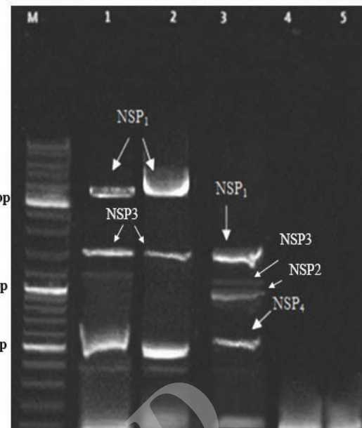
Figure 5. Demonstration of Poly (A) RT-PCR amplification of normal and rearranged rotavirus in 1% agarose gel. Lane 1 & 2) amplification of rearranged rotavirus; Lane 3) normal rotavirus; Lane 4) mir48 as positive control. Lane 5) negative control. M: Mix molecular weight marker.
