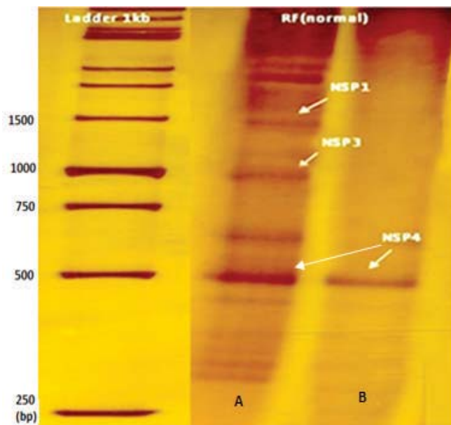
Figure 4. Demonstration of Poly (A) RT-PCR reaction. Normal rotavirus profile in 10% polyacrylamide gels and silver staining.
