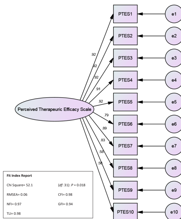
Figure 1. Confirmatory Factor Analysis of the Perceived Therapeutic Efficacy Scale.
