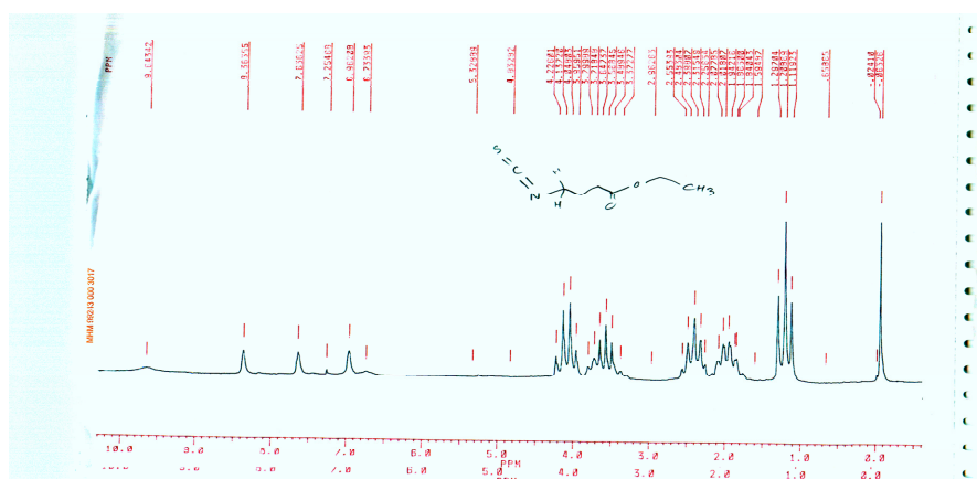
Fig. 2- NMR spectra of ethyl 4-isothiocyanatobutyrate (ETCB)
