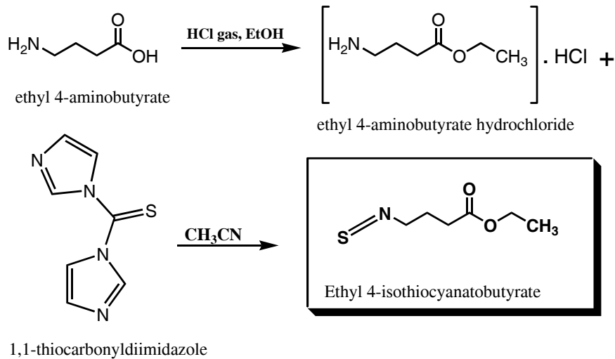
Fig. 1- Synthetic procedure of Ethyl 4-isothiocyanatobutyrate
