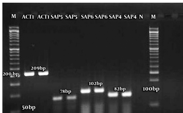
Figure 1. The Electrophoresis Product of RT-PCR on SAP4-SAP6 and ACT1 Genes
