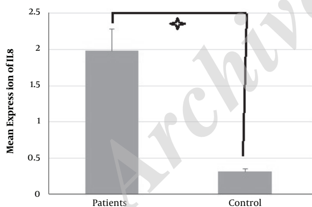
Figure 5. Comparison of mRNA expression levels of IL-8 in patients and healthy controls in human peripheral blood mononuclear cells analyzed by the real-time PCR; significant differences at P < 0.05 .
