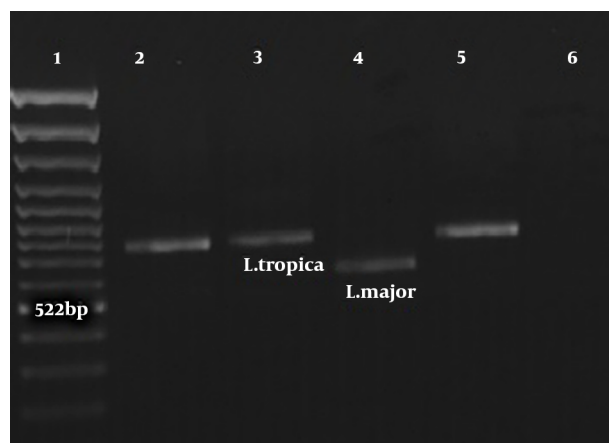
Figure 4. Lanes 1, ladder 100 pb; lane 2, L. tropica (positive control); Lane 3 and 5, L. tropica , lane 6: negative control; lane 4, L. major .
