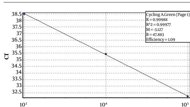
Figure 3. Representative standard curves for IL-23 using the Light Cycler device. All samples are shown in duplicate.
