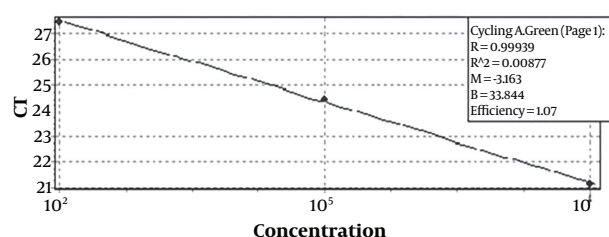
Figure 1. Representative standard curves for the \beta 2M gene using the Light Cycler device
