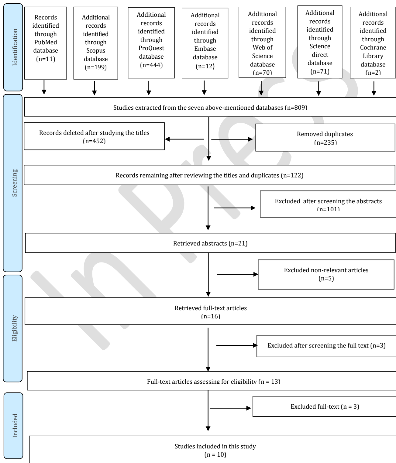
Figure 1. Preferred reporting item for systematic reviews and meta-analyses flow diagram of screened papers
