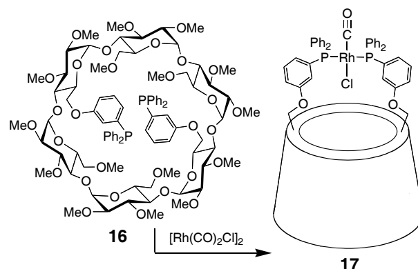
Scheme 6. Synthesis of a hydroformylation catalyst based on a cyclodextrin-modified diphosphine.
