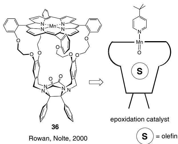
Scheme 12. Olefin epoxidation catalyst based on a molecular clip.
