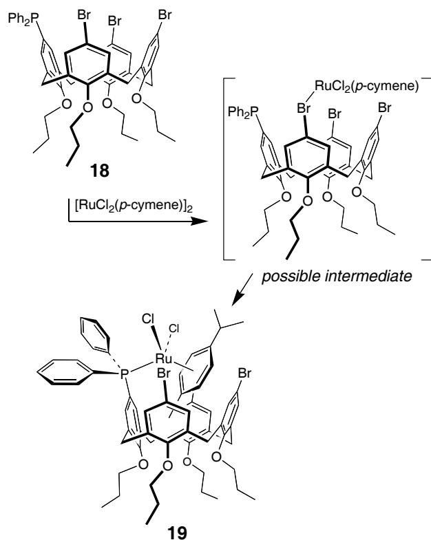
Scheme 7. Filling the calixarene basket with an organometallic ruthenium unit.
