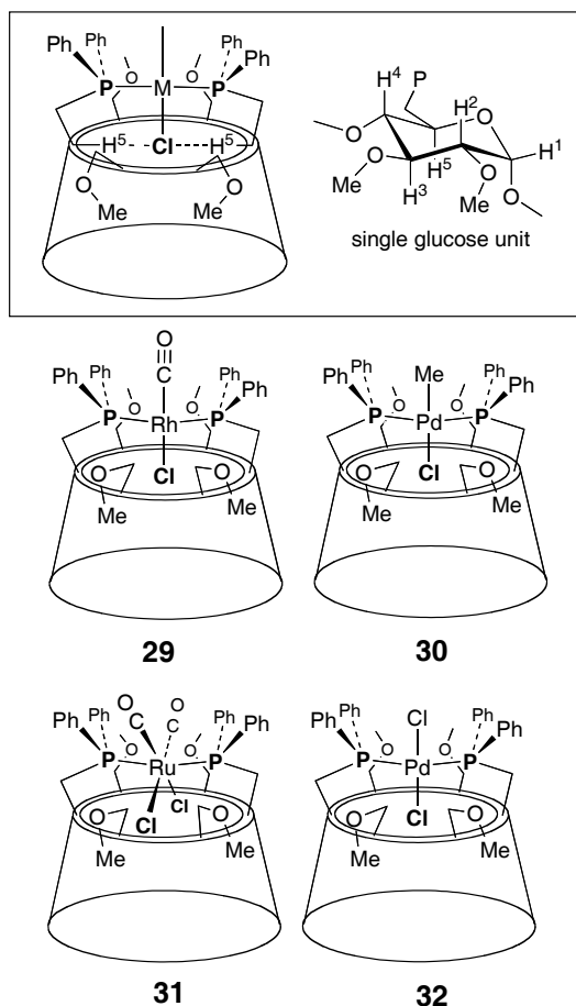
Fig. 2. Weak Cl...cavity interactions (involving H 5 atoms) in metallo-cyclodextrins.
