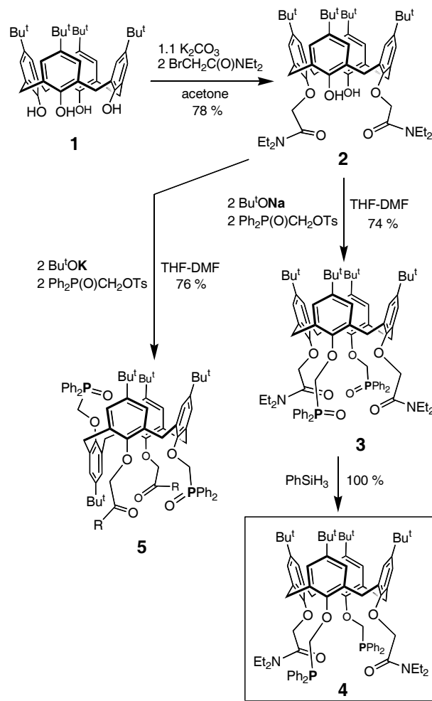
Scheme 1. Synthesis of diphosphine 4.
