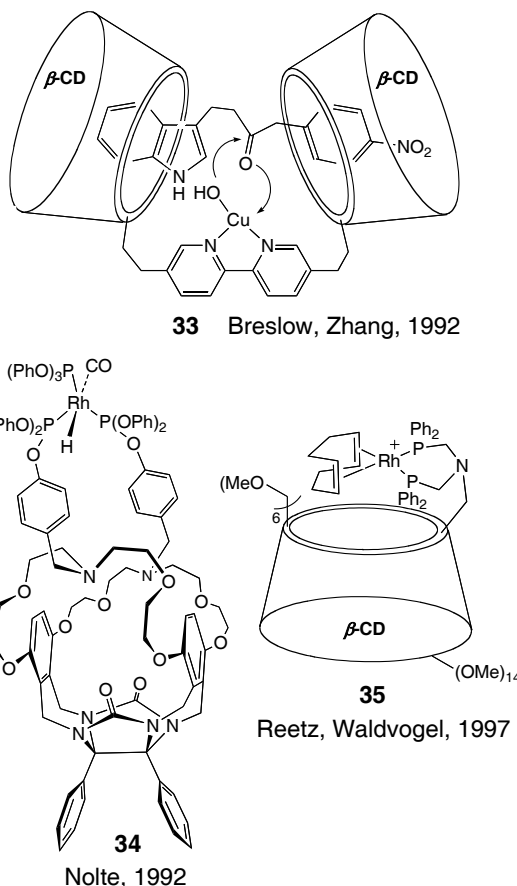
Fig. 3. Supramolecular catalysts based on a cavitant ( 33 , 35 ) or a molecular clip ( 34 ).
