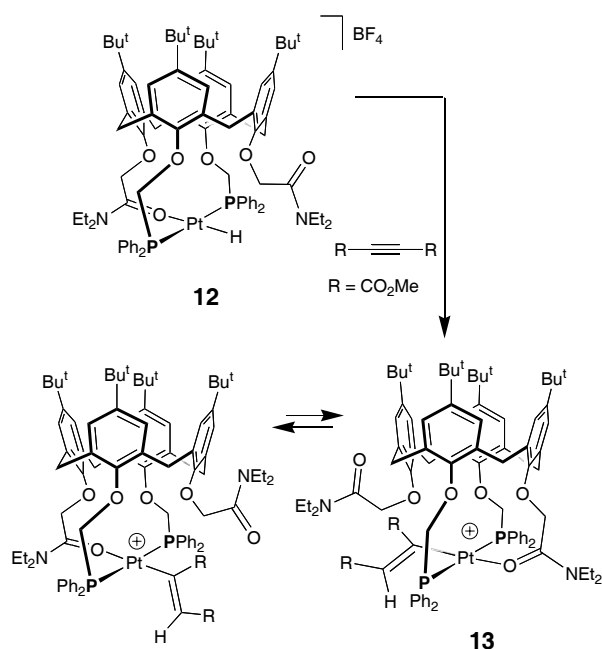
Scheme 4. Reactivity of a semi-encapsulated platinum hydride.
