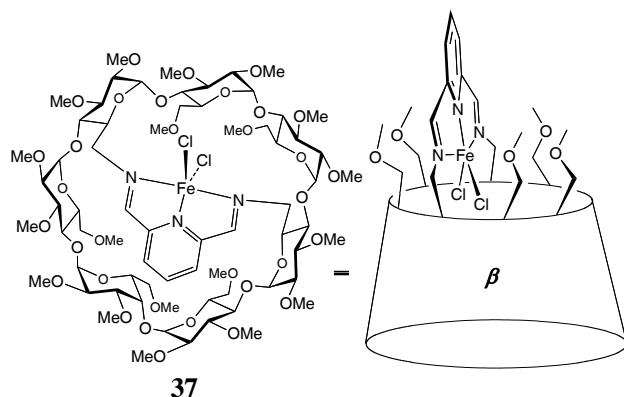
Fig. 4. The first polymerization catalyst operating in a "tube".
