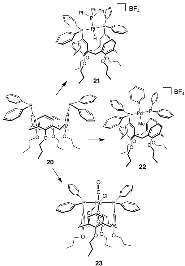
Scheme 8. Confinement of metal-organic fragments in the calix[4]arene 20 .
