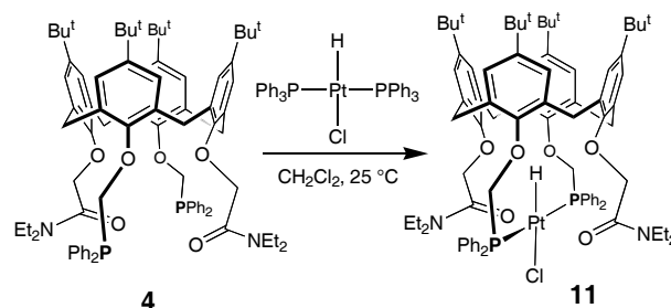
Scheme 3. Confinement of a Pt-H bond at the narrow entrance of a calix[4]arene.
