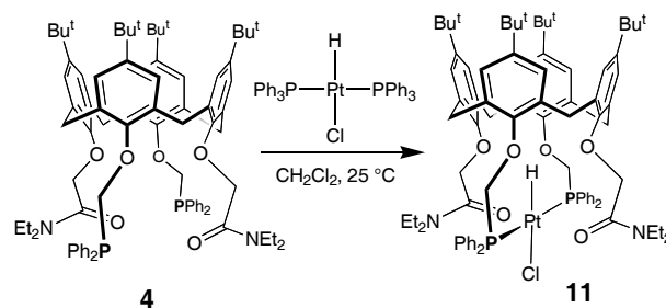
Scheme 3. Confinement of a Pt-H bond at the narrow entrance of a calix[4]arene.
