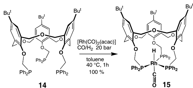
Scheme 5. Controlling the orientation of a "H-Rh-CO" rod.
