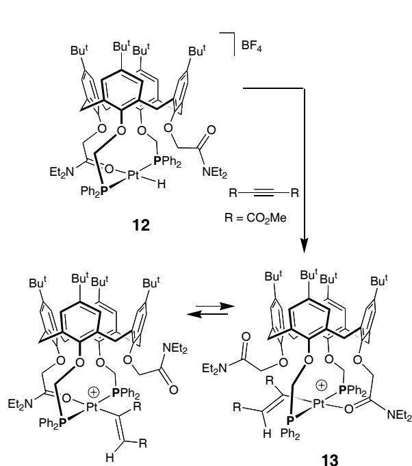
Scheme 4. Reactivity of a semi-encapsulated platinum hydride.
