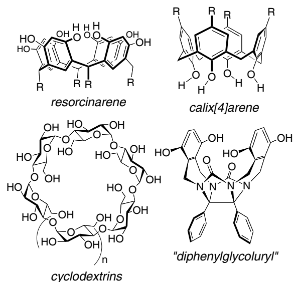
Fig. 1. Most employed procavittands.
