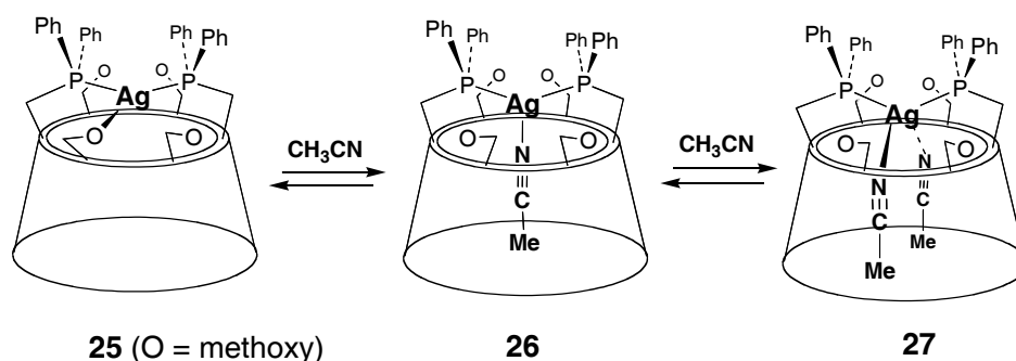
Scheme 11. Coordination chemistry inside a cyclodextrin cavitand.
