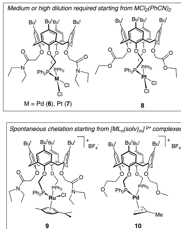
Scheme 2. Calix[4]arene chelate complexes in which the metal centre is positioned at the lower rim.
