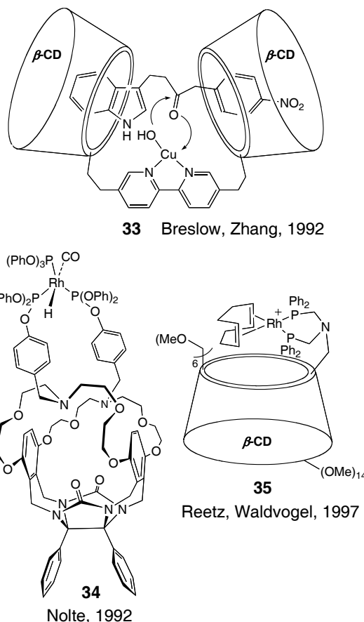
Fig. 3. Supramolecular catalysts based on a cavitand ( 33 , 35 ) or a molecular clip ( 34 ).
