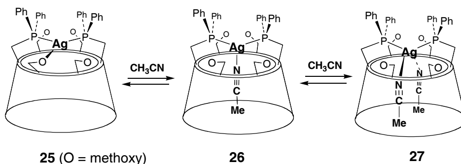
Scheme 11. Coordination chemistry inside a cyclodextrin cavitation.
