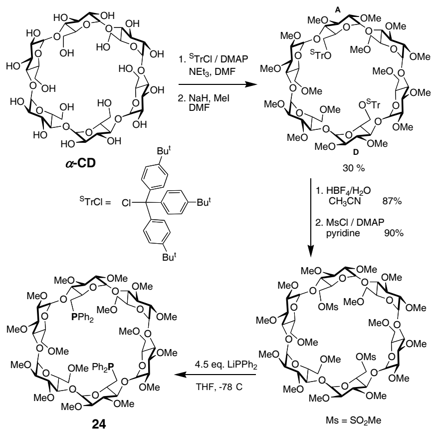
Scheme 9. Synthesis of the cyclodextrin diphosphine 24 .
