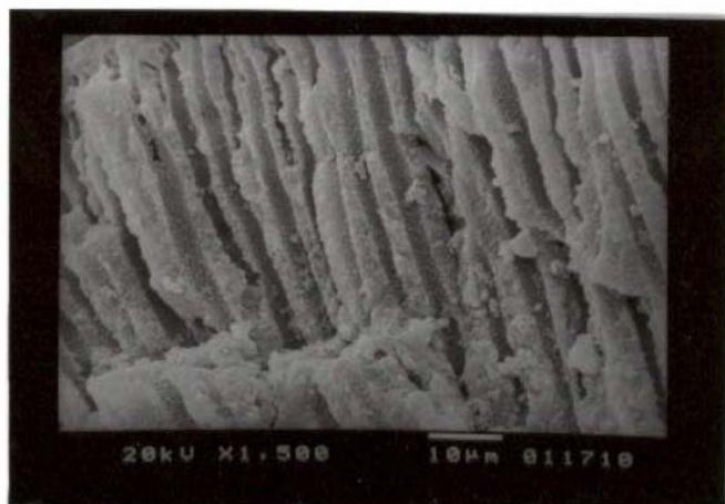
Fig. 7. Scanning electron micrograph of the digested material (Ordered-Porous titanium phosphate).
