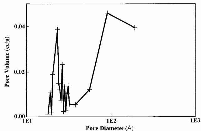
Fig. 6. BJH pore size distribution plot for the digested material calculated from desorption branch of the isotherm plot.
