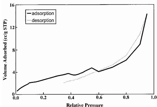
Fig. 5. Adsorption-desorption isotherm plot of digested material.
