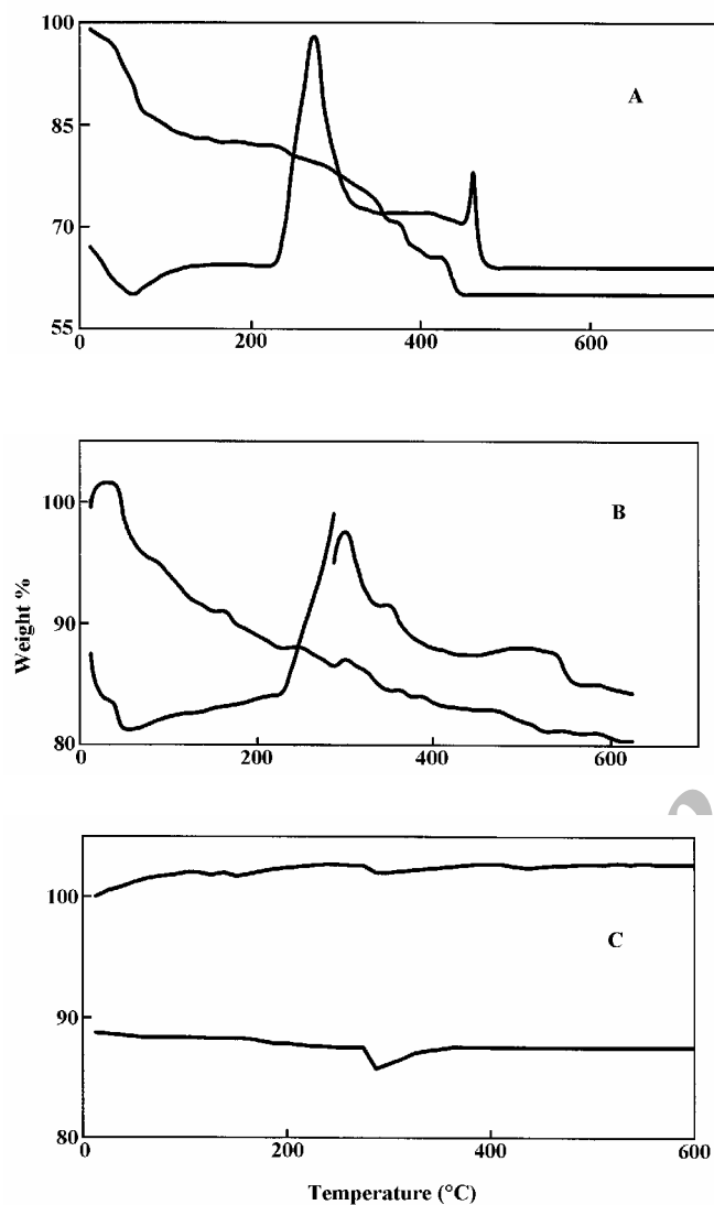
Fig. 2. TGA-DTA curves of primary (precursor) product (A), digested (surfactant-titanium phosphate) material (B) and calcined precursor material (C).
