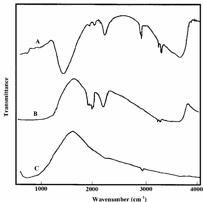
Fig. 1. FTIR spectra of surfactant-titanium phosphate product (A), primary (precursor) product (B) and calcined propoxide precursor (C).
