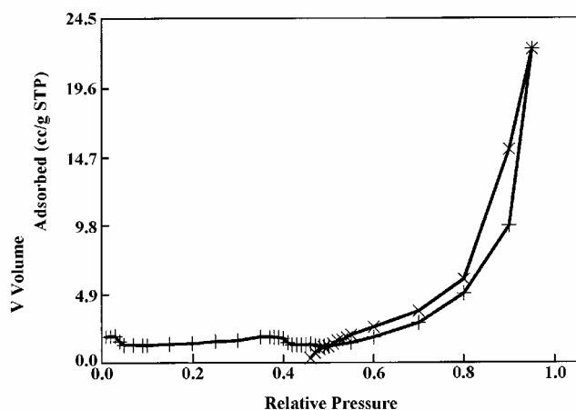
Fig. 4. Nitrogen sorption isotherm plot of digested material at 77 K.
