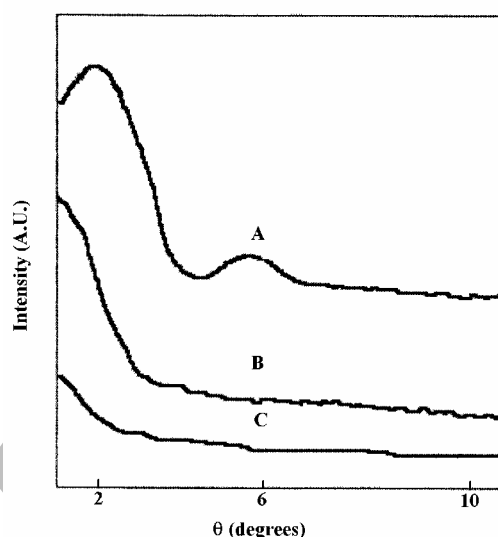
Fig. 3. XRD patterns of surfactant-titanium phosphate product (A), primary (precursor) product (B) and calcined precursor material (C).
