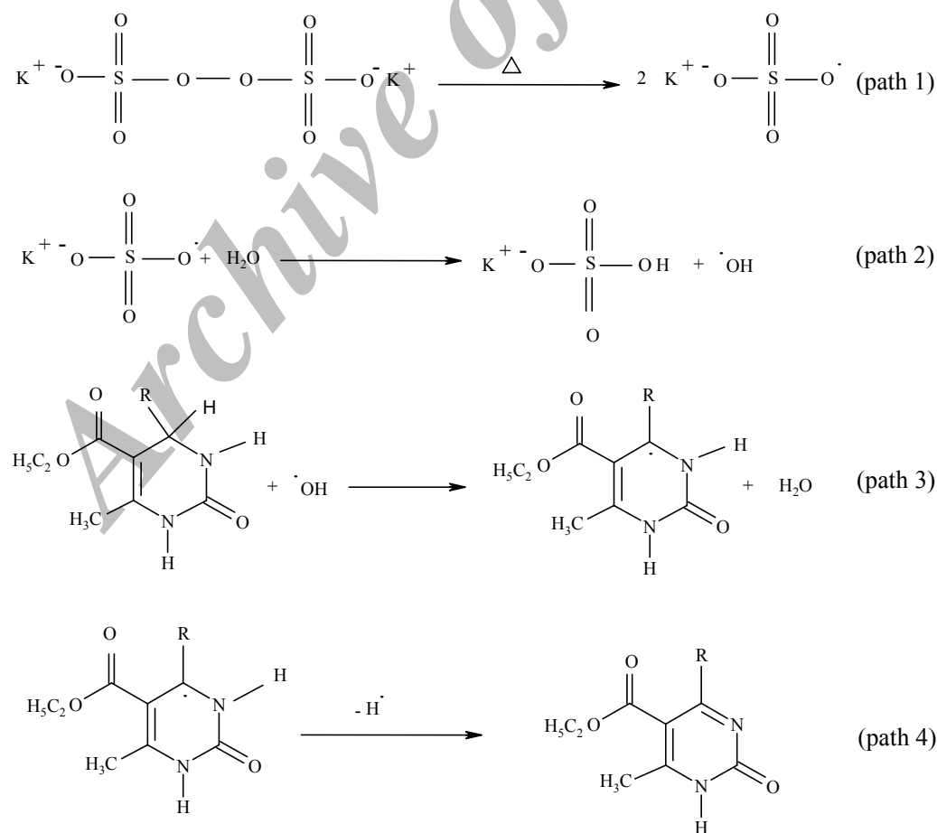
Scheme 3. Proposed mechanism for dehydrogenation of DHPMs by \text{K}_2\text{S}_2\text{O}_8
