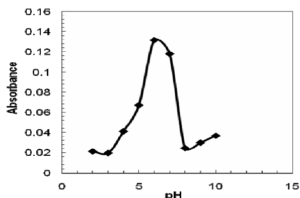
Fig. 2. Effect of pH on calibration curve. Conditions: wavelength of measurement; 270 nm, volume of buffer solution; 2.0 ml; HCT concentration, 3.0\ \mu\text{g}\ \text{ml}^{-1} .
