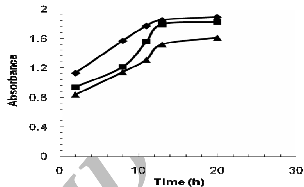
Fig. 3. Optimization of solvent ratio and time extraction. Conditions: volume of extraction solvent, 150 \text{ ml} ; wavelength of measurement, 270 \text{ nm} : (◆) methanol-acetic acid 9:1, v/v; (■) methanol-acetic acid 7:3, v/v; (▲) methanol-acetic acid 5:5, v/v.
