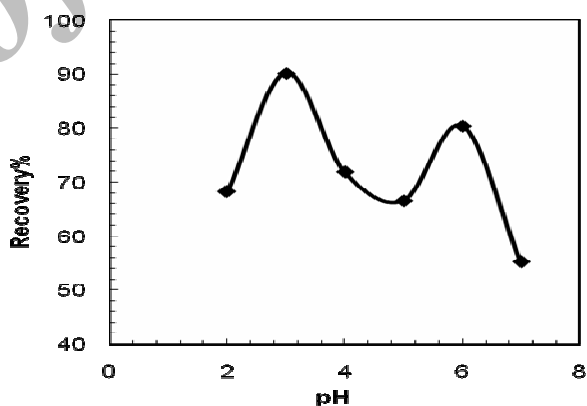
Fig. 4. Effect of pH on the adsorption efficiency. Conditions: column packing material, 200 \text{ mg} ; buffer solutions volume, 2.0 \text{ ml} ; HCT concentration, 30.0 \mu\text{g ml}^{-1} ; flow rate, 0.554 \text{ ml min}^{-1} ; wavelength of measurement, 270 \text{ nm} .
