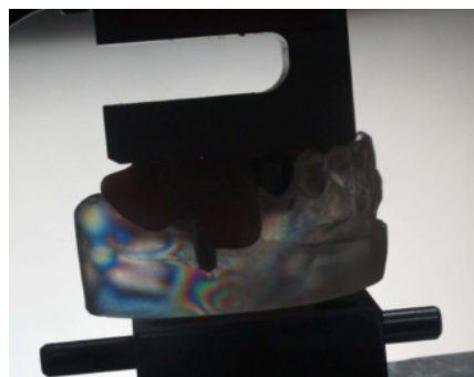
Figure 8. Photoelastic analysis
