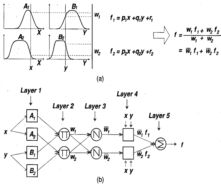
FIGURE 3. (a) A two input first order Sugeno fuzzy model with two rules, (b) Equivalent ANFIS architecture.
