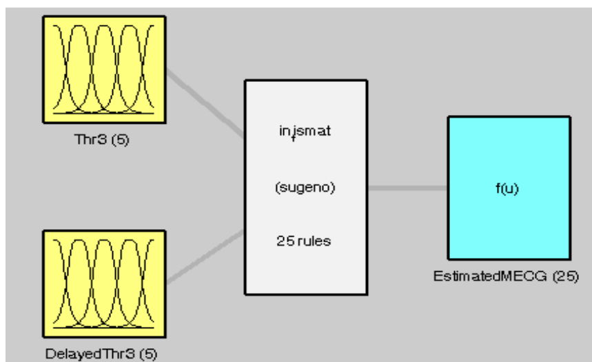
FIGURE 7. Fuzzy model generated by GENFIS.
