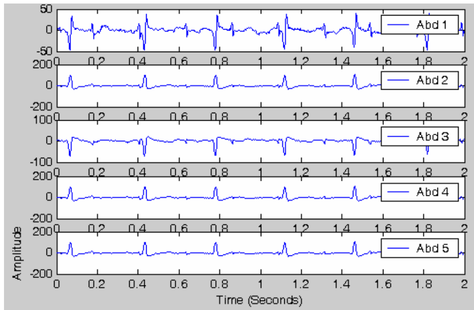
FIGURE 4. Abdominal signals from different electrode positions.
