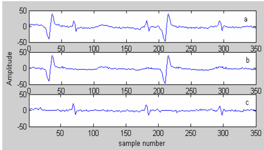
FIGURE 10. (a) Abd1 containing non overlapping three FECG beats and two MECG beats, (b) Estimated MECG (c) the extracted FECG.
