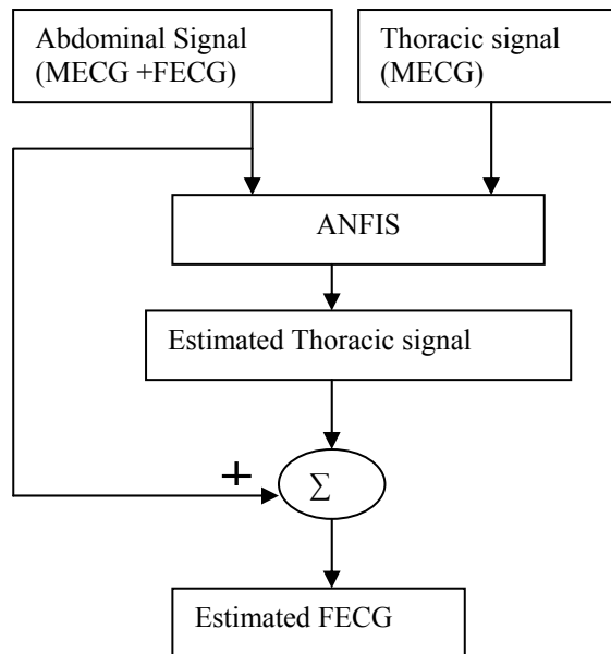
FIGURE 6. Flowchart for the cancellation of MECG and the extraction of FECG.
