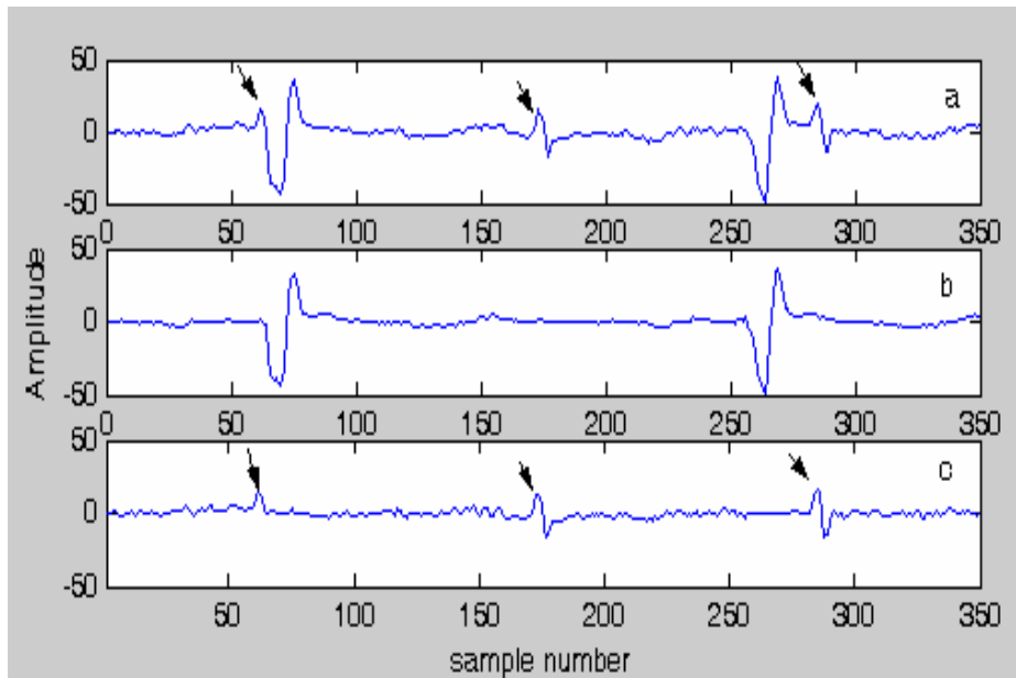
FIGURE 12. (a) Abd1 containing full overlap between the first FECG beat and the MECG, (b) Estimated MECG (c) the extracted FECG signal.
