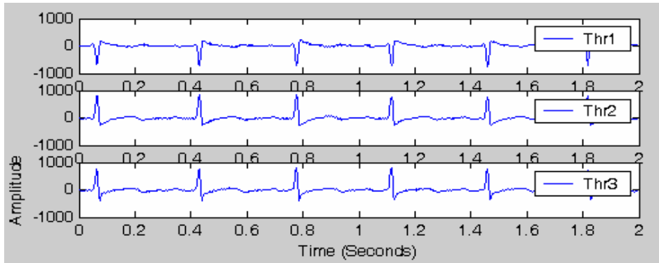
FIGURE 5. MECG signals measured at the thorax region of a pregnant woman.
