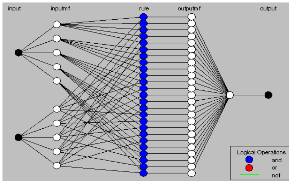
FIGURE 8. ANFIS structure.
