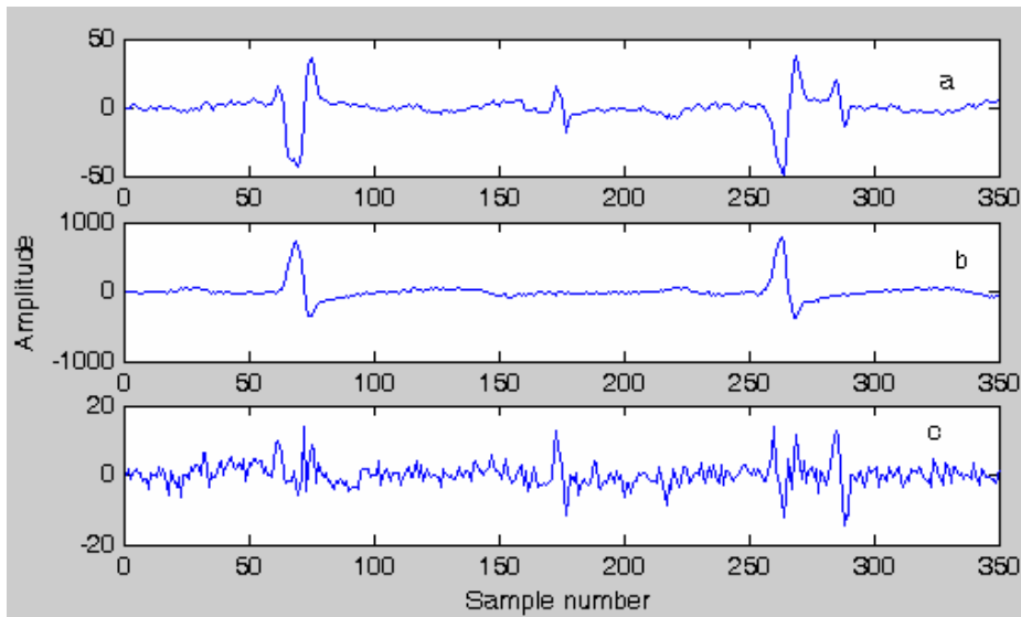
FIGURE 13. FECG extraction using back propagation neural network.
