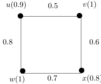
Figure 1: Illustration of Strong Coverings in Fuzzy Graphs
