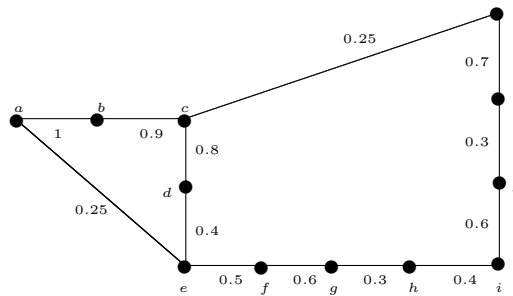
Figure 5: Illustrating that \gamma_{spr} > \gamma_{sc}
