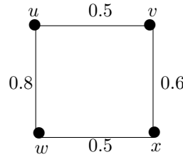
Figure 4: Private Strong Dominating Set
