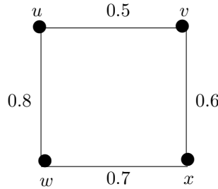
Figure 3: Illustration of strong paired domination
