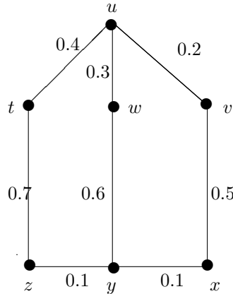
Figure 5: Illustrating that \gamma_{spr} > \gamma_{sc}
