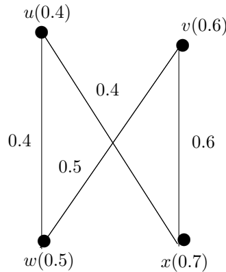
Figure 2: Perfect Strong Matching
