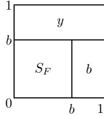
Figure 1: F in Theorem 3.3(ii)
