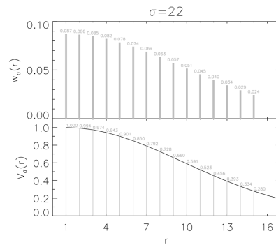
Figure 2: The Infinite Gaussian maxitive OWA weights function and Infinite Gaussian OWA weights function with parameter \sigma_4 = 22 .
