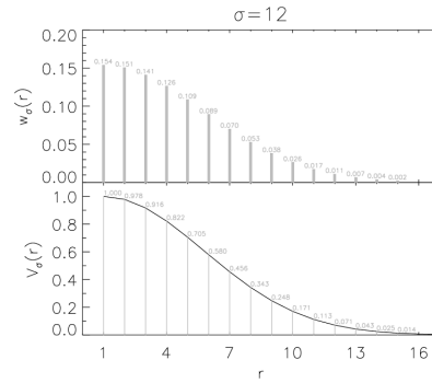
Figure 1: The Infinite Gaussian maxitive OWA weights function and Infinite Gaussian OWA weights function with parameter \sigma_2 = 12 .
