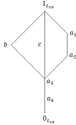
Figure 10: The lattice L_{10}
