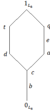
Figure 6: The lattice L_6
