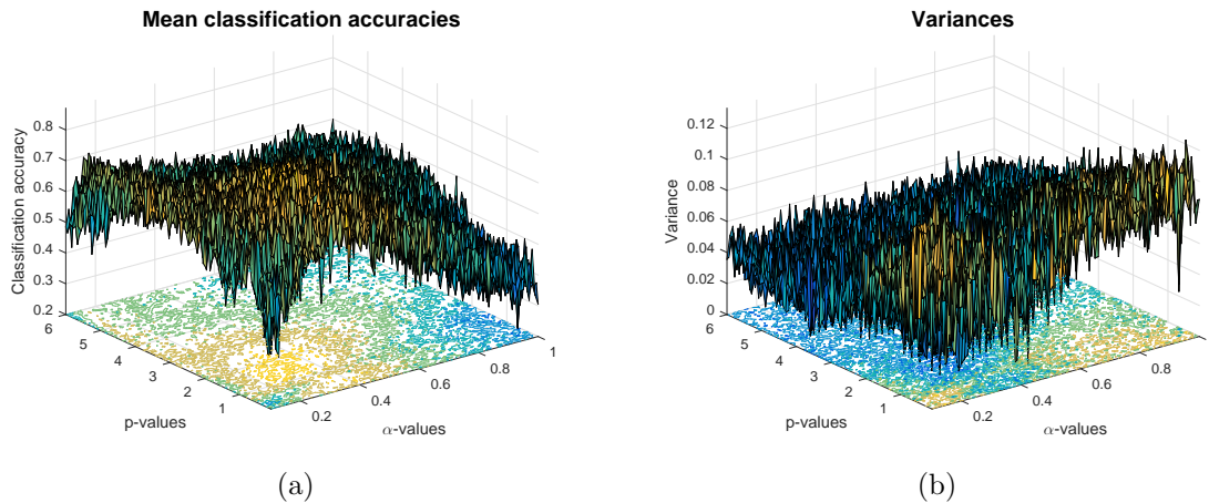
Figure 2: Mean classification accuracies (a) and the variances (b) obtained from fertility data set with generalized Heronian mean at q = 12 .
