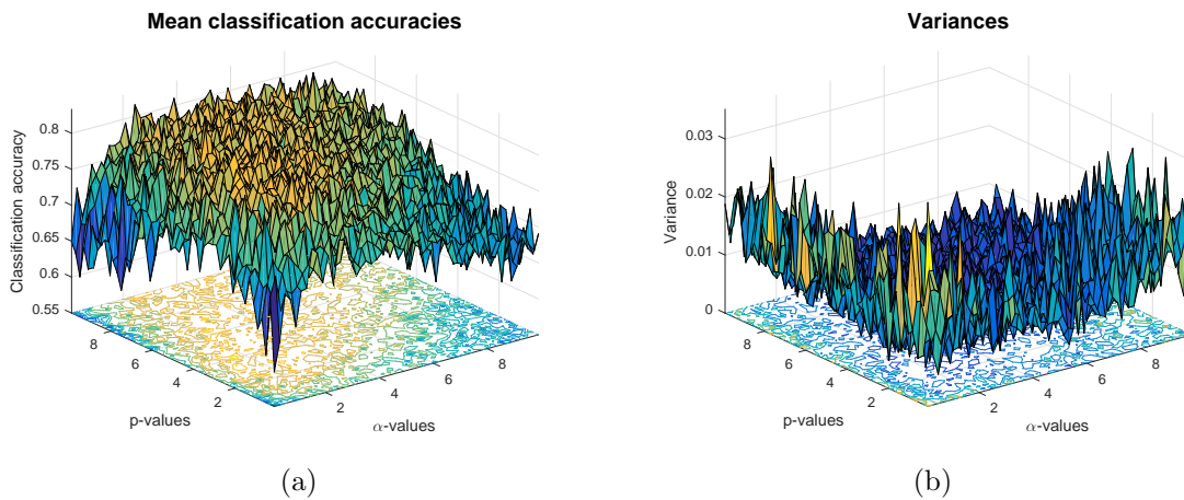
Figure 4: Mean classification accuracies (a) and the variances (b) obtained from lung cancer data set with generalized Heronian mean at q = 5 .
