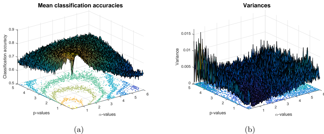
Figure 1: Mean classification accuracies (a) and the variances (b) obtained from echocardiogram data set with generalized Heronian mean at q = 0.5 .
