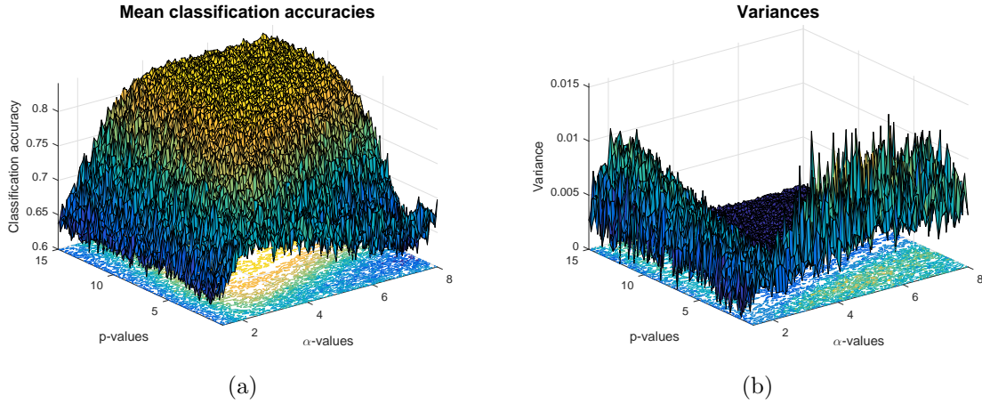
Figure 3: Mean classification accuracies (a) and the variances (b) obtained from horse-colic data set with generalized Heronian mean at q = 5 .
