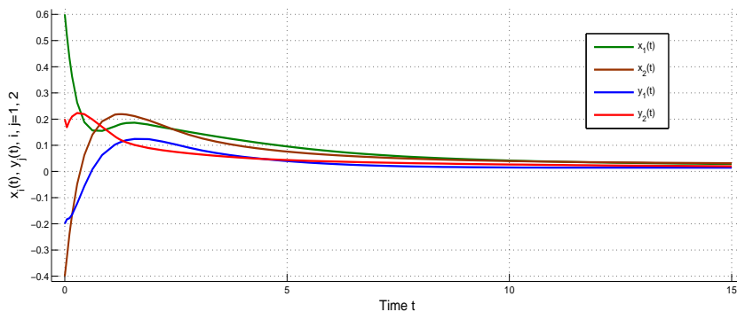
Figure 1: State trajectories of the FBAMNNs (21) in Example 4.1
